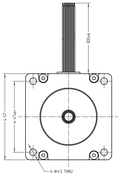
Mechanical View 1
