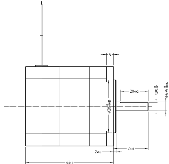
Mechanical View 2
