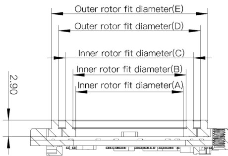
Mechanical View 1
