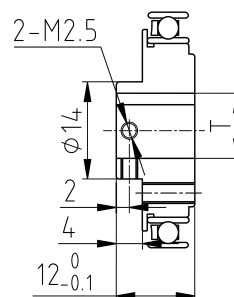
Mechanical View 6
