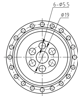
Mechanical View 2
