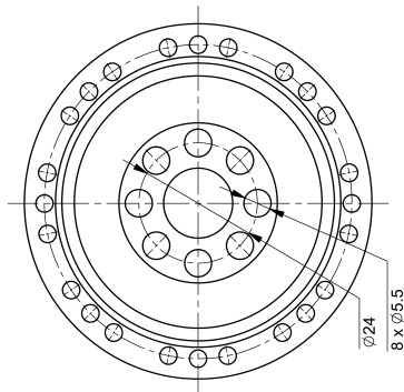
Mechanical View 3
