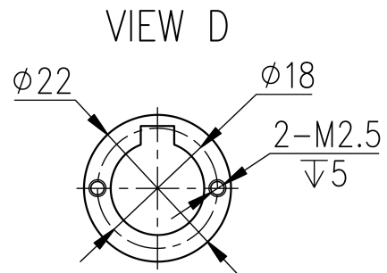
Mechanical View 4
