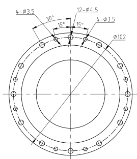
Mechanical View 1
