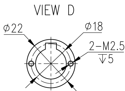
Mechanical View 4
