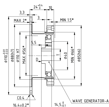
Mechanical View 2
