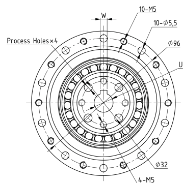
Mechanical View 2
