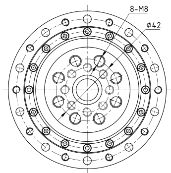
Mechanical View 3
