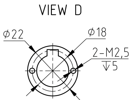
Mechanical View 4
