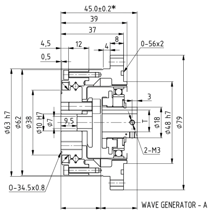
Mechanical View 1
