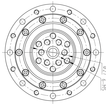
Mechanical View 2
