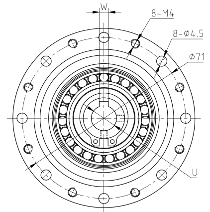
Mechanical View 3
