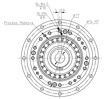
Mechanical View 3
