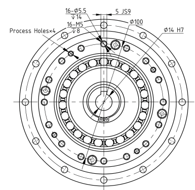
Mechanical View 3
