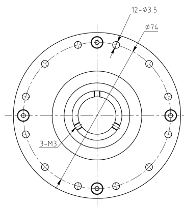
Mechanical View 2
