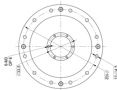
Mechanical View 2
