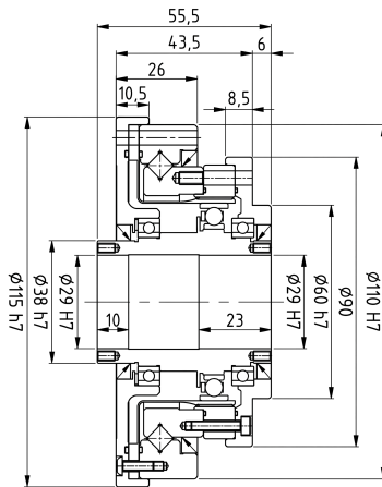
Mechanical View 1
