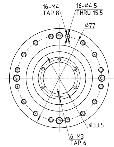
Mechanical View 3
