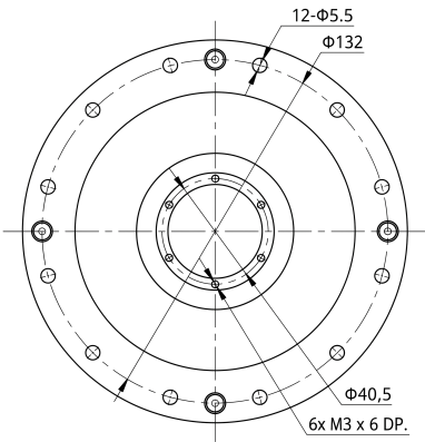
Mechanical View 2
