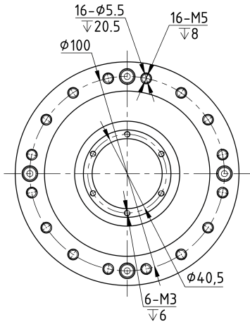
Mechanical View 3
