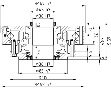
Mechanical View 1
