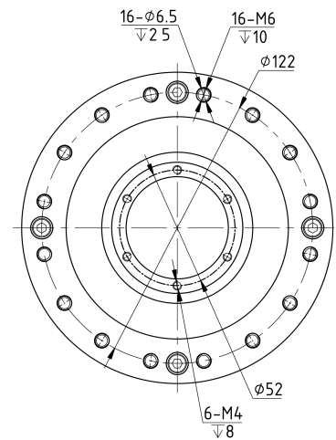
Mechanical View 3
