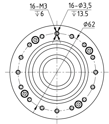
Mechanical View 3
