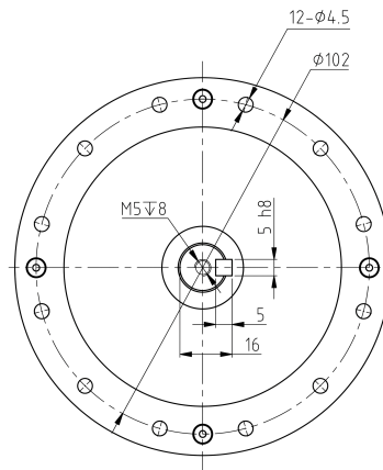
Mechanical View 2
