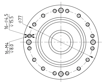
Mechanical View 3
