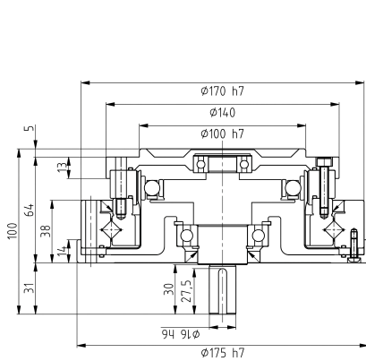
Mechanical View 1
