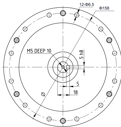
Mechanical View 2
