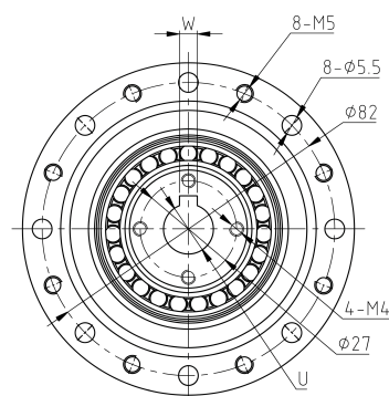
Mechanical View 2
