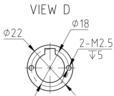
Mechanical View 4
