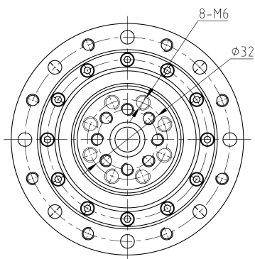
Mechanical View 3
