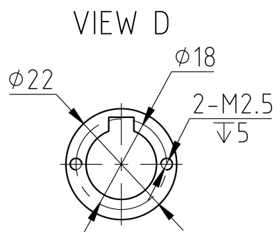
Mechanical View 4
