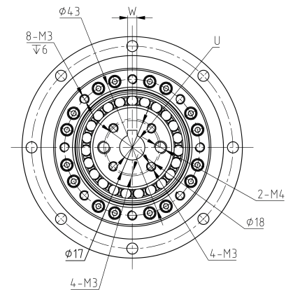
Mechanical View 3
