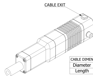
Mechanical View 5
