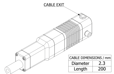
Mechanical View 5
