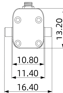
Mechanical View 2
