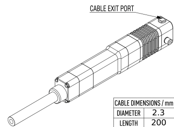
Mechanical View 5
