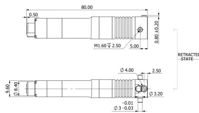
Mechanical View 4
