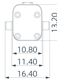
Mechanical View 2
