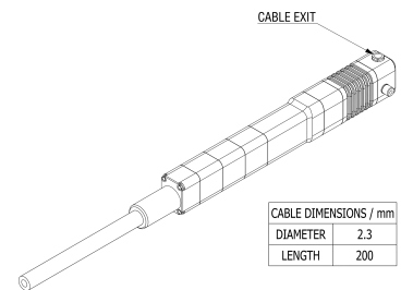
Mechanical View 5
