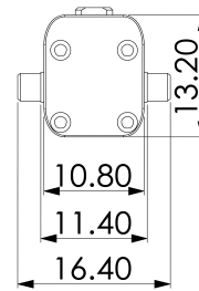
Mechanical View 2
