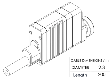
Mechanical View 4
