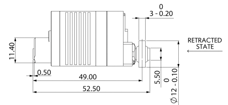
Mechanical View 5
