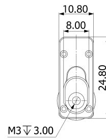
Mechanical View 2
