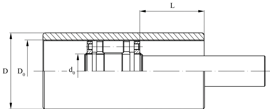
Mechanical View 1
