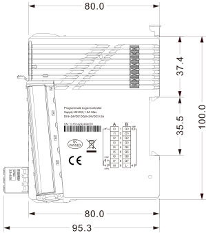
Mechanical View 2
