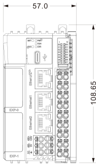
Mechanical View 4
