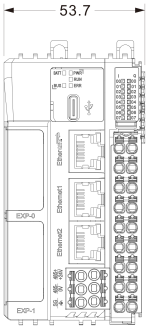
Mechanical View 1
