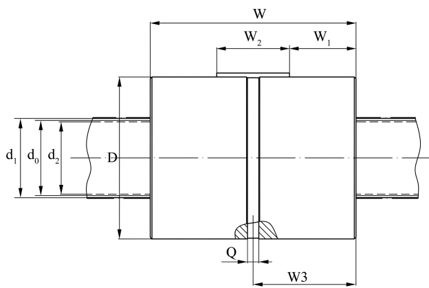
Mechanical View 1
