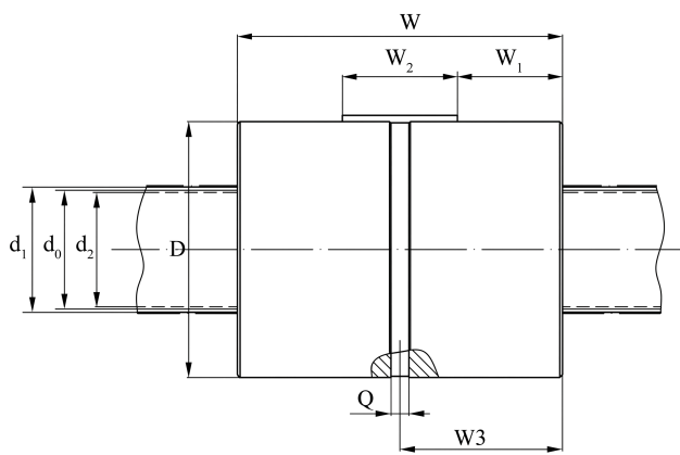
Mechanical View 1
