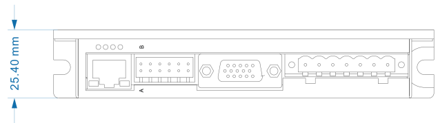
Mechanical View 2
