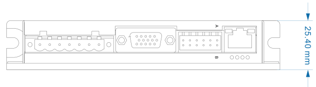
Mechanical View 2
