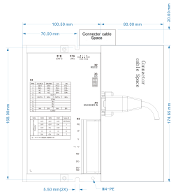
Mechanical View 1
