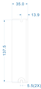
Mechanical View 3
