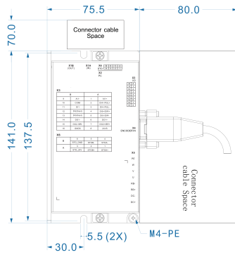
Mechanical View 1
