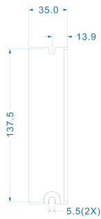
Hole position for fixation Mechanical View 3
