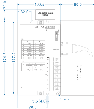
Mechanical View 1
