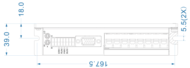
Mechanical View 2
