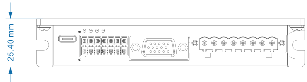
Mechanical View 2
