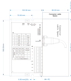
Mechanical View 1
