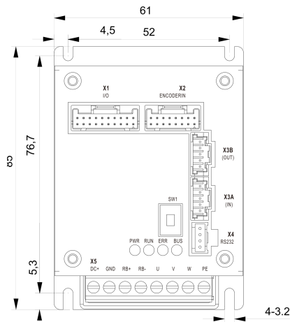
Mechanical View 2
