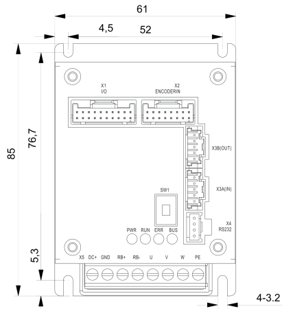
Mechanical View 2
