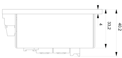
Mechanical View 1
