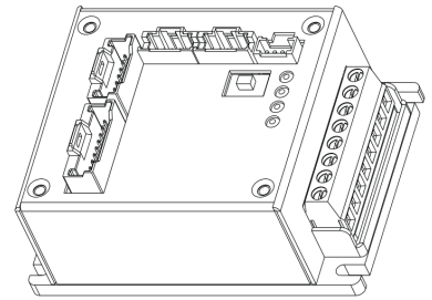
Mechanical View 3
