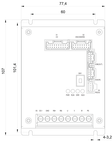
Mechanical View 1
