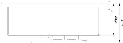
Mechanical View 2
