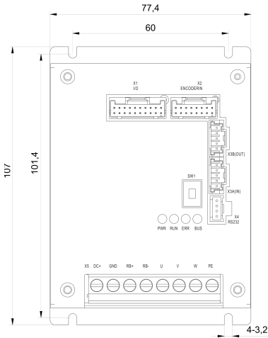
Mechanical View 1
