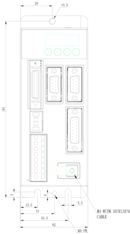
Mechanical View 1
