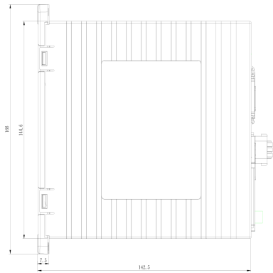
Mechanical View 3
