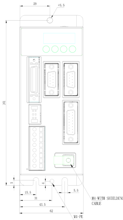
Mechanical View 1
