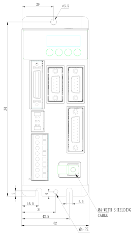
Mechanical View 1
