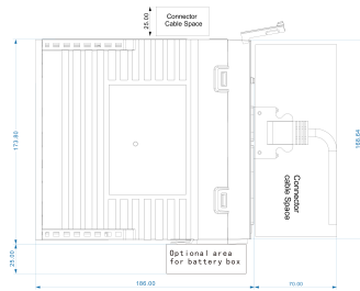
Mechanical View 1
