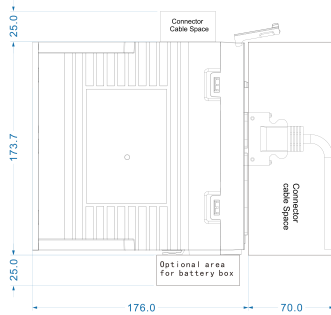
Mechanical View 1
